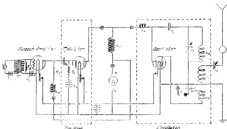
FIG. 14 - 200 Watt Constant Current Transmitter
